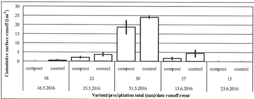
Fig. 4 Surface runoff in 2016 – spring barley
