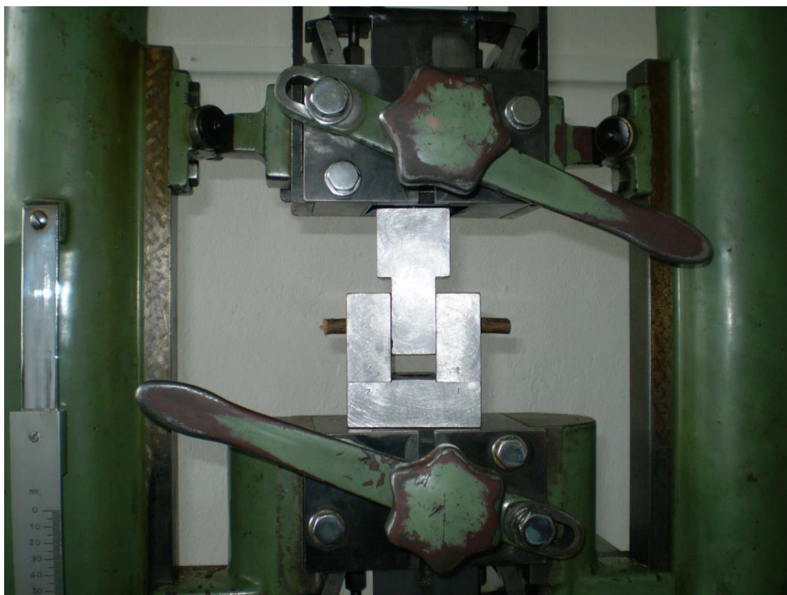
Figure 1. Adapter (jig) for measurement of shear stress limit
