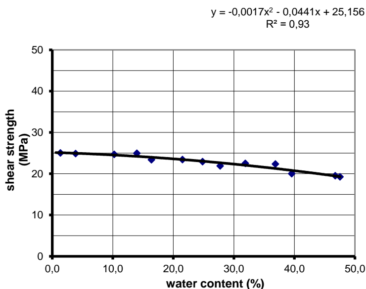
Figure 3. Course of shear strength limit in dependence on all water content – willow
