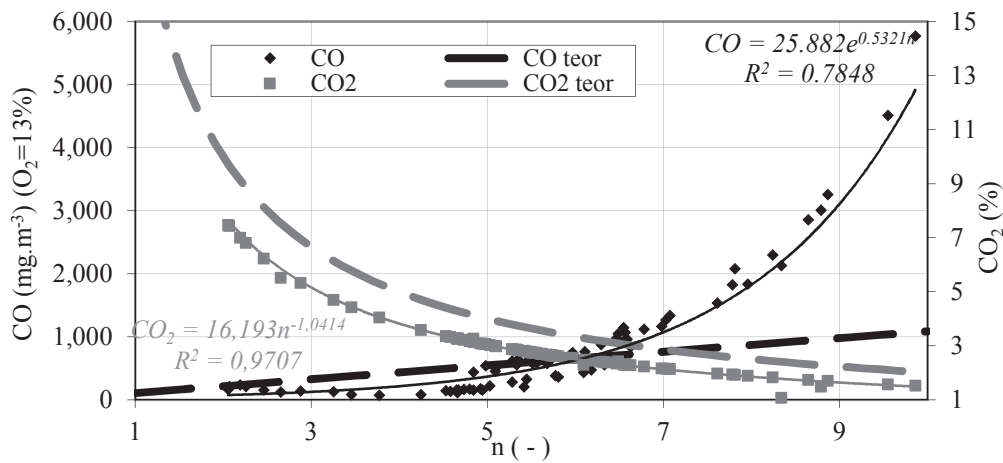
Figure 1. Theoretical and real dependence of carbon monoxide and carbon dioxide on the excess air coefficient – combustion of briquettes from compost.
