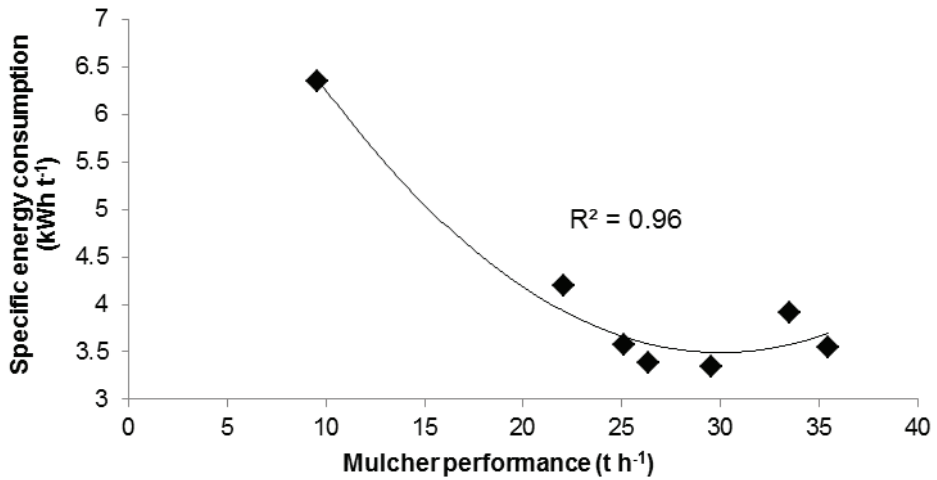
Figure 2. Specific energy consumption of the mulcher.
