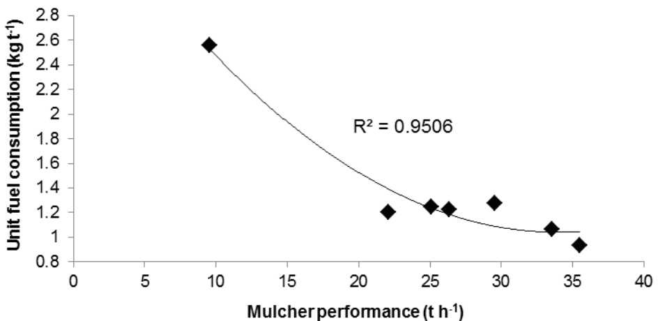
Figure 3. Unit fuel consumption.
