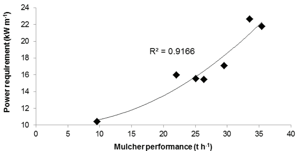
Figure 1. Mulcher power requirement.
