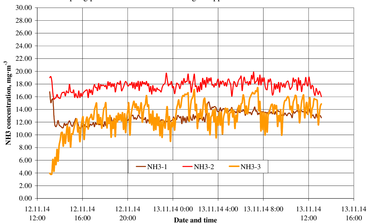
Fig. 3. Ammonia concentration in the hall No. 1
