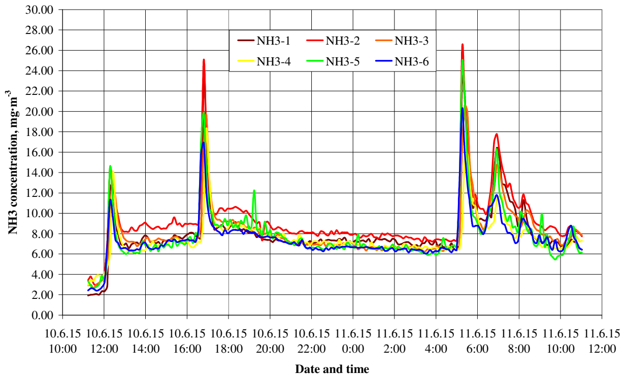
Fig. 2. Ammonia concentration in the hall 9A
