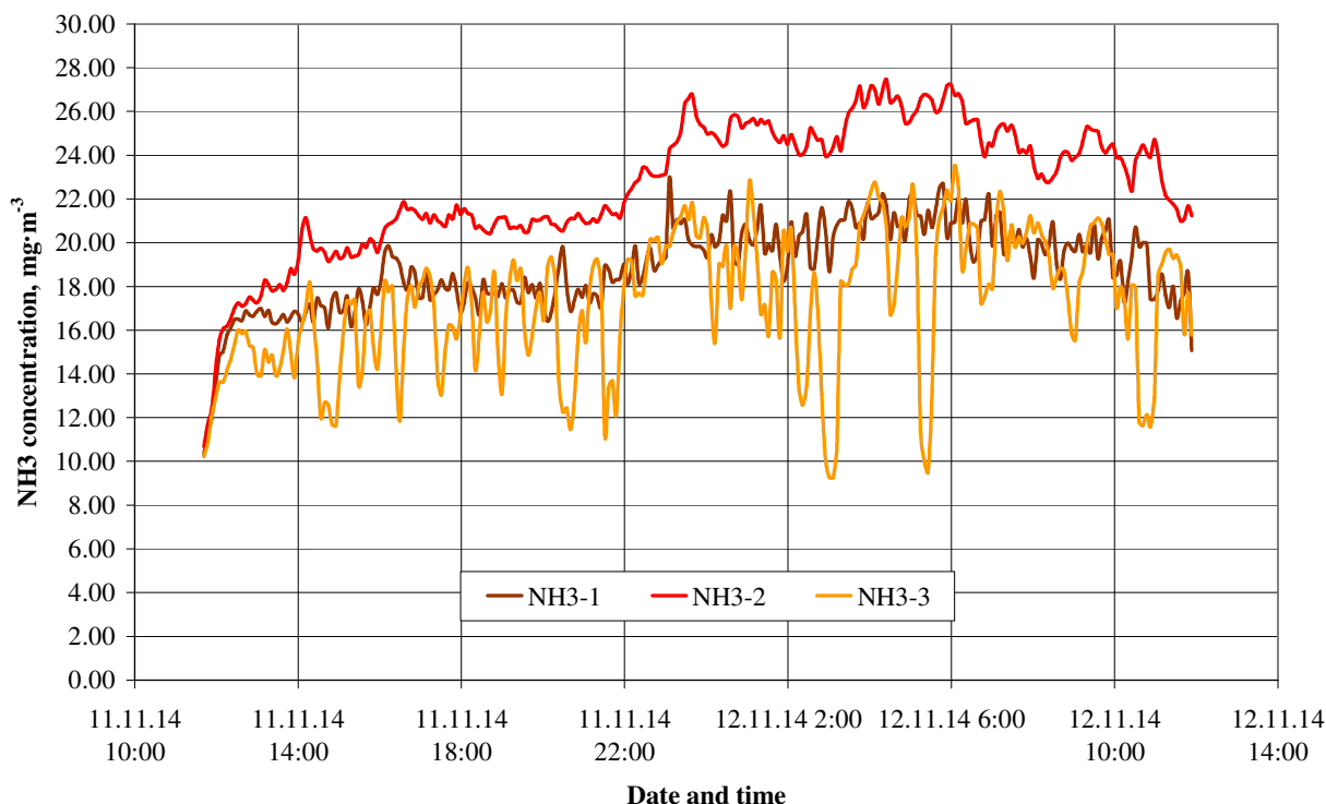
Fig. 4. Ammonia concentration in the hall No. 2
