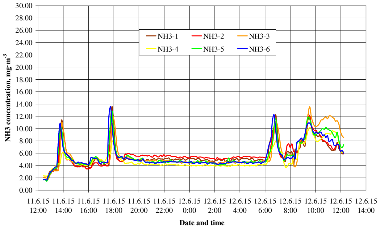
Fig. 1. Ammonia concentration in the hall 10D
