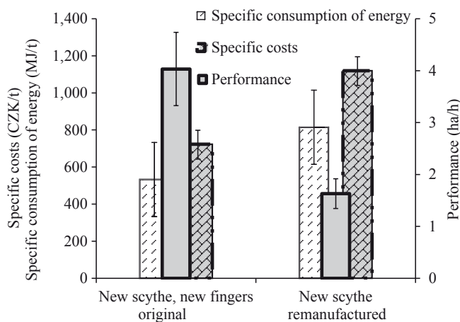
Fig. 3. Dependence of performance, specific energy consumption and specific costs of linseeds harvesting on cutting mechanism condition
