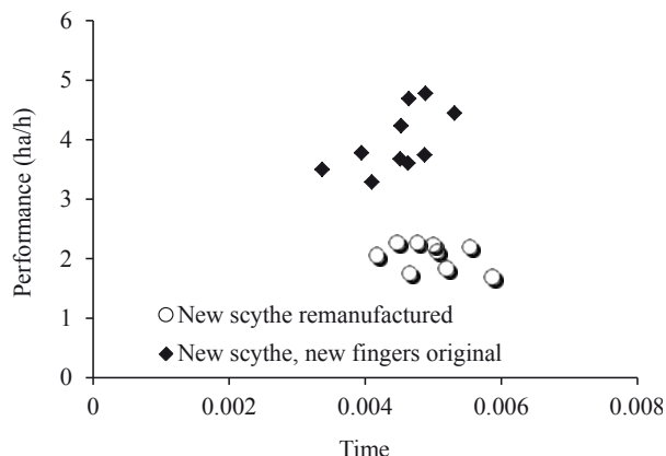
Fig. 1. Dependence of performance on cutting mechanism condition
