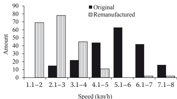
Fig. 2. Working speeds histogram
